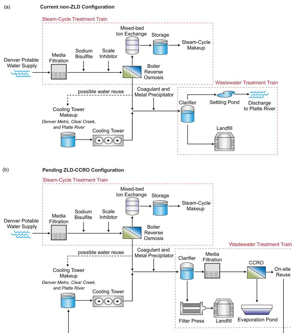
Figure 4. Process flow diagram showing water treatment for Cherokee Generating Station's (a) current, non-ZLD configuration and (b) pending ZLD-CCRO configuration. The Steam-Cycle Treatment Train treats Cherokee's steam-cycle water, and the Wastewater Treatment Train treats both the steam-cycle RO concentrate and cooling-cycle blowdown water. Flow rates are reported in Table S1, source water constituents are reported in Table S2, and water-recovery and constituent-removal rates are reported in Table S4.
