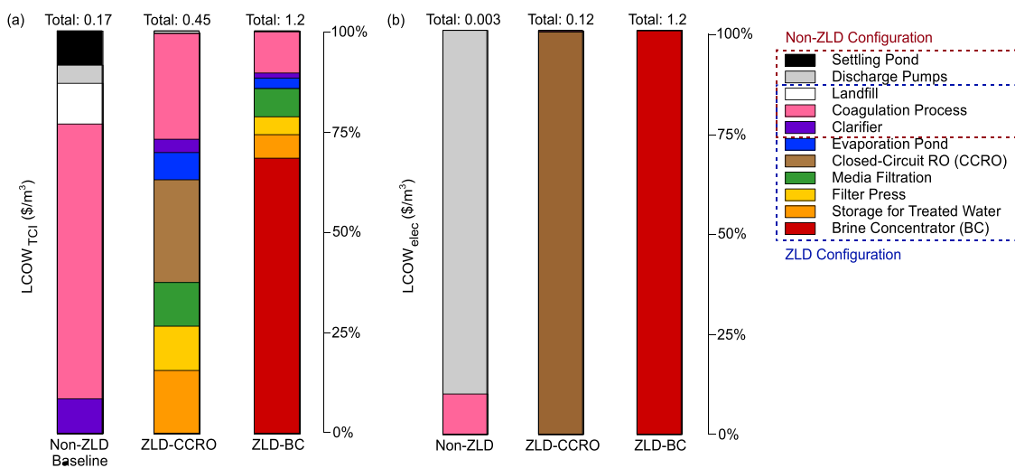
Figure 7. (a) LCOW_{TCI} (as given by eq 3 and shown by the red bars of Figure 6) and (b) LCOW_{elec} (as given by eq 8 and shown by the green bars of Figure 6) broken down by individual treatment processes/units at the Cherokee Generating Station. The units/processes included in the non-ZLD baseline configuration are boxed by the red-dashed line in the legend and the units/processes included in the ZLD configurations are boxed by the blue-dashed line in the legend. LCOW values for the two ZLD scenarios are compared with the non-ZLD baseline scenario. To discern between the processes/units that have smaller contributions to LCOW_{TCI} and LCOW_{elec} , the y axes are given in percentages (from 0 to 100%). The total LCOW for each scenario is given at the top of each bar.
