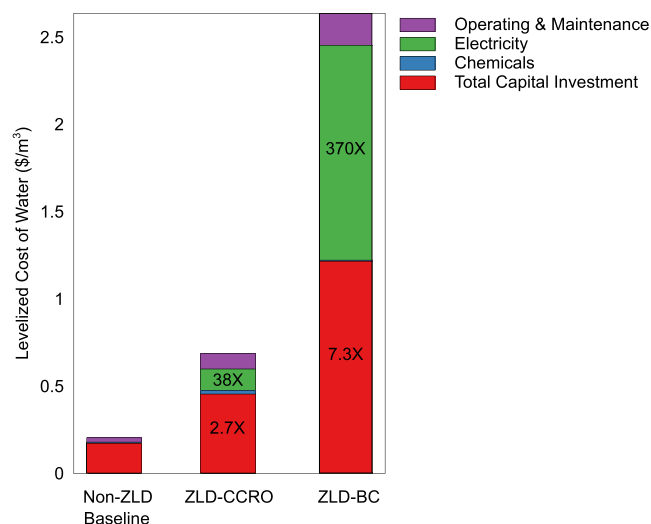
Figure 6. Levelized cost of water (LCOW) for the two ZLD scenarios (ZLD-CCRO and ZLD-BC) are compared with LCOW for the non-ZLD baseline scenario for Cherokee Generating Station. LCOW values are broken down into general cost categories. Further breakdown of the cost categories (i.e., detail of the \text{LCOW}_{\text{TCI}} and \text{LCOW}_{\text{elec}} values) is shown in Figure 7.
