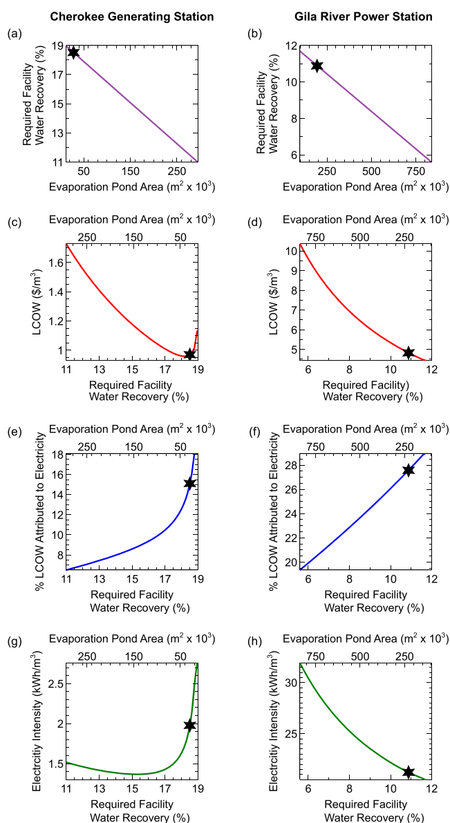
Figure 10. Relationship between required facility water recovery and evaporation pond area for (a) Cherokee Generating Station and (b) Gila River Power Station. Analyses evaluating the impact of facility water recovery and evaporation pond area on (c) Cherokee's LCOW, (d) Gila's LCOW, (e) Cherokee's percent LCOW attributed to electricity, (f) Gila's percent LCOW attributed to electricity, (g) Cherokee's electricity intensity, and (h) Gila's electricity intensity. The black stars indicate the existing evaporation pond areas for Cherokee (28 300 m 2 ) and Gila (194 250 m 2 ); the corresponding facility water recoveries (18.5% for Cherokee and 11.4% for Gila) were used in the modeling.
