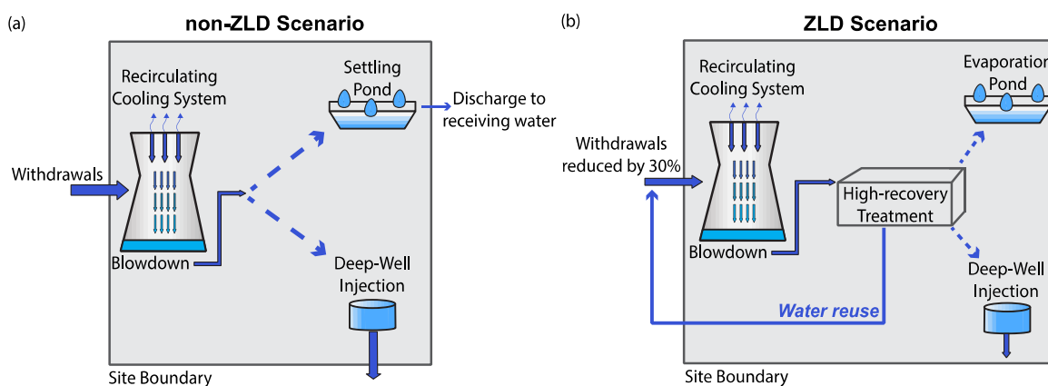
Figure 2. Schematic of water balance at power facilities (a) without a ZLD system and (b) with a ZLD system. A power facility without a ZLD system can treat cooling tower blowdown with a settling pond before discharge to a receiving water or can discharge directly to a deep well. A power facility with a ZLD system treats cooling tower blowdown with a high-recovery treatment system. The product water can be reused for cooling tower makeup (or other upstream uses), which reduces withdrawal requirements. The residual from the high-recovery treatment system can either be discharged to an on-site evaporation pond or injected in a deep well.
