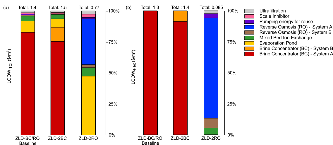
Figure 9. (a) LCOW_{TCI} (as shown in eq 3 and red bars in Figure 8) and (b) LCOW_{elec} (as shown in eq 8 and green bars in Figure 8) broken down by individual treatment processes/units at Gila River Power Station. LCOW values for the two alternative ZLD scenarios are compared with the ZLD-BC/RO baseline scenario. To discern between the processes/units that have smaller contributions to LCOW_{TCI} and LCOW_{elec} the y axes are given in percentages (from 0 to 100%). The total LCOW for each scenario is given at the top of each bar, are still discernible.
