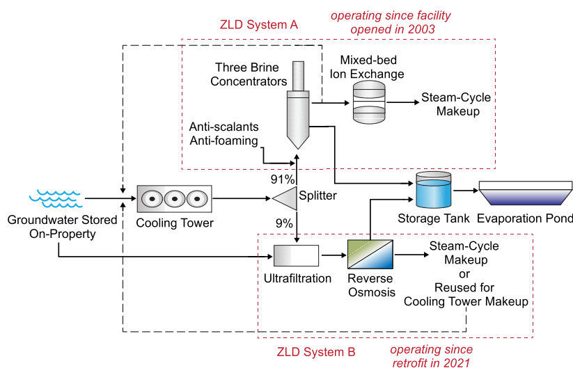
Figure 5. Gila River Power Station process flow diagram. The cooling towers use groundwater that is stored on-site. Cooling tower blowdown water is treated with ZLD System A or ZLD System B before it is reused for cooling tower makeup or steam-cycle makeup. ZLD System A treats the majority of cooling tower blowdown water (modeled as 91% in this study) and is composed of three brine concentrators followed by mixed-bed ion exchange. ZLD System B treats a smaller fraction of the cooling tower blowdown water (modeled as 9% in this study) and is composed of ultrafiltration and reverse-osmosis processes. Concentrate from ZLD System A and ZLD System B is combined in a storage tank before discharge to on-site evaporation ponds. Flow rates are reported in Table S1, source water constituents are reported in Table S2, and water-recovery and constituent-removal rates are reported in Table S4.
