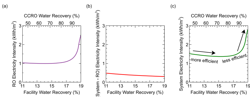
Figure 11. Relationship between electricity intensity and facility recovery for Cherokee Generating Stations' (a) CCRO process and (b) all processes/units in ZLD system aside from CCRO (c) the overall ZLD system.
