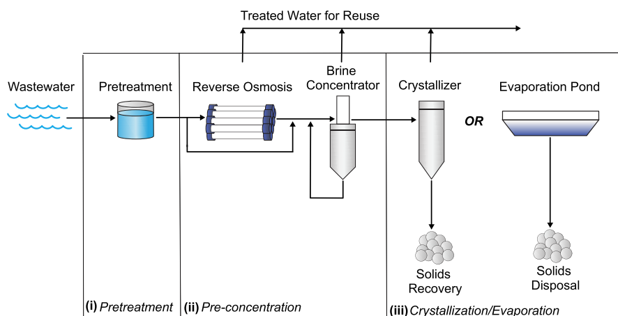
Figure 3. Conventional zero liquid discharge (ZLD) treatment scheme with (i) pretreatment, (ii) preconcentration by reverse osmosis and/or a brine concentrator, and (iii) crystallization/evaporation by crystallizers and/or evaporation ponds. Figure adapted from Global Water Intelligence. 93
