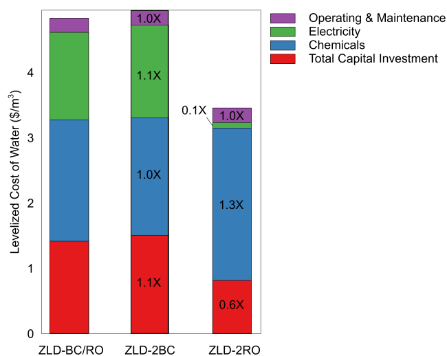
Figure 8. Levelized cost of water (LCOW) for the two alternative ZLD scenarios (ZLD-2BC and ZLD-2RO) compared with LCOW for the ZLD-BC/RO baseline scenario for Gila River Power Station. LCOW values are broken down into general cost categories. Further breakdown of the cost (i.e., detail of the \text{LCOW}_{\text{TCI}} and \text{LCOW}_{\text{elec}} values) is shown in Figure 9.
