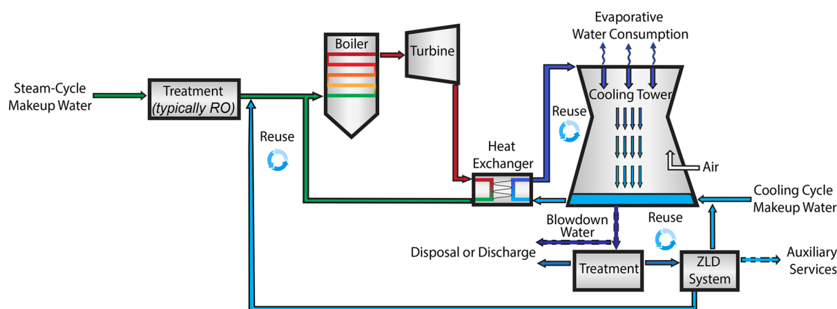
Figure 1. Water flow diagram of a thermoelectric power facility with a recirculating cooling tower and a ZLD system. Water reuse occurs in the cycles of concentration of the cooling tower. Water reuse also occurs when ZLD systems typically installed to meet discharge regulations provide high-quality effluent that is recycled back to the facility.
